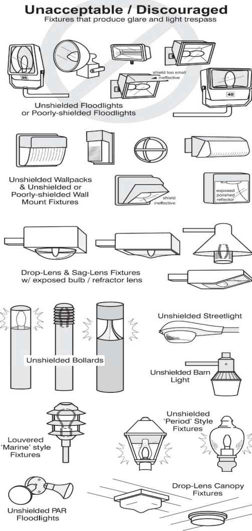
FIGURE 52-403M: ACCEPTABLE/UNACCEPTABLE LIGHTING FIXTURES
